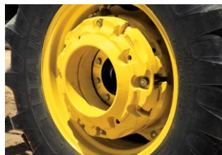
Add more traction. T19293 Rear wheel weights
