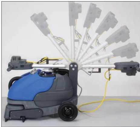
Adjustable folding handle for comfort and storage.
